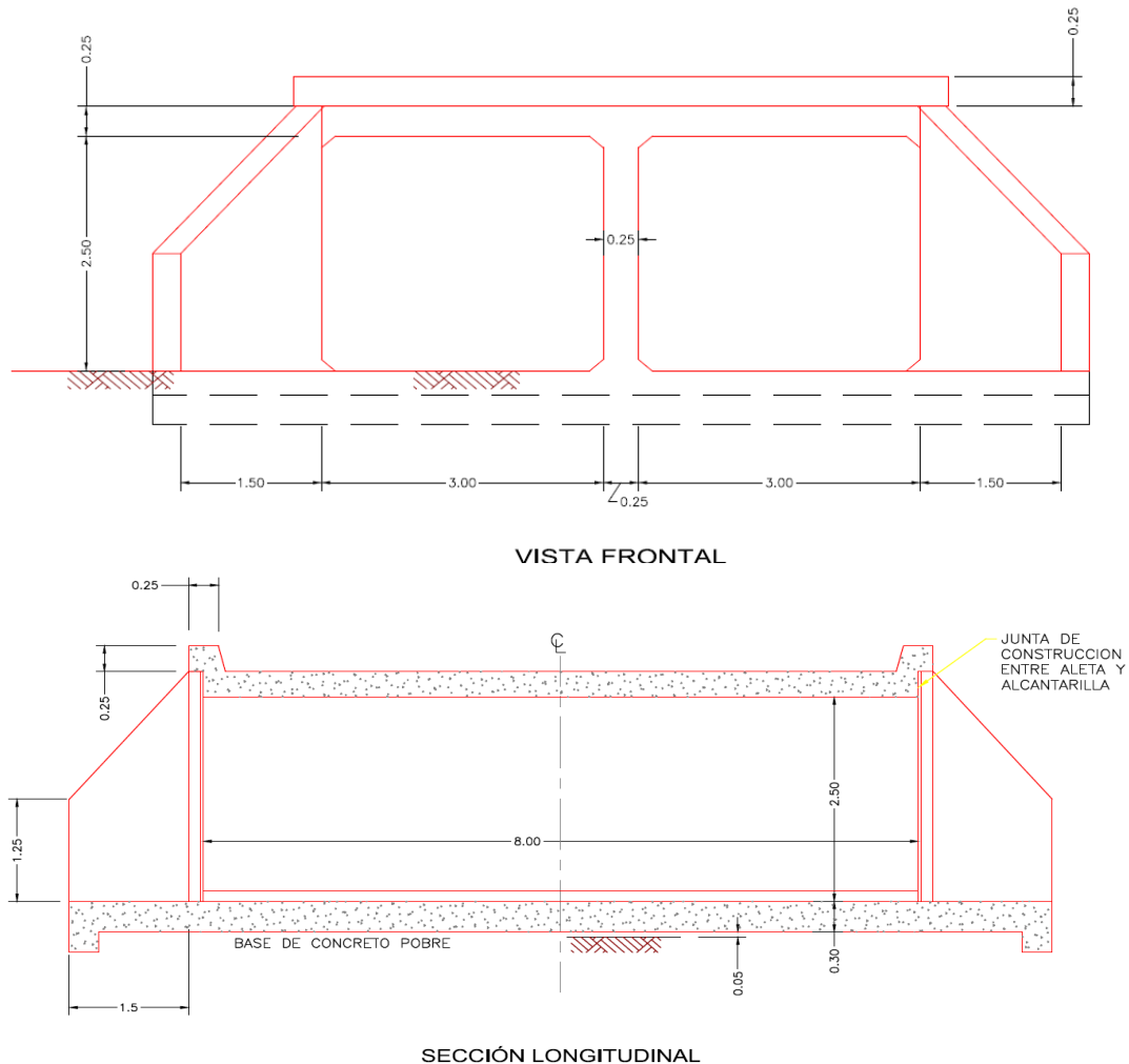
Figura 2-51 Box culvert
